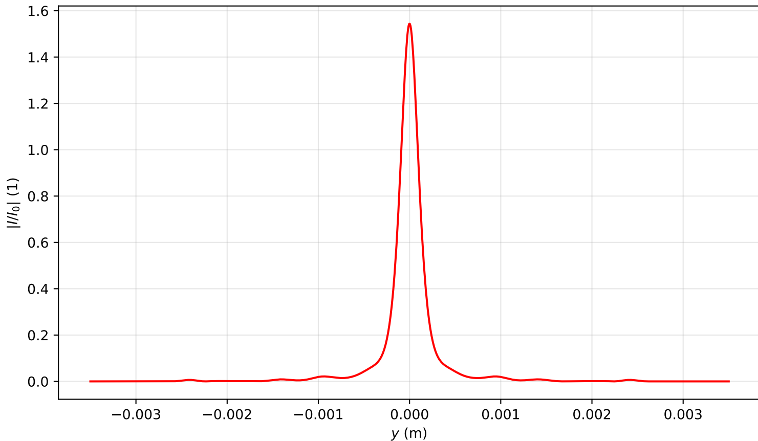
Intensity profile I(x=0, y, z=3.184)/I_0 , P_{in}=4.0P_{cr} , artificial time
